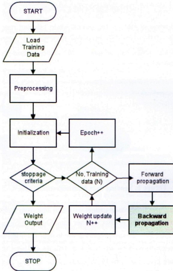
Figure 2. Block diagram of learning process.
