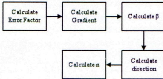
Figure 3. Backward propagation in learning process.
